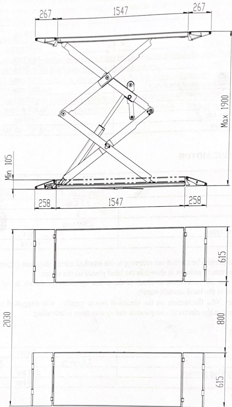
Figure 2 – LAYOUT
